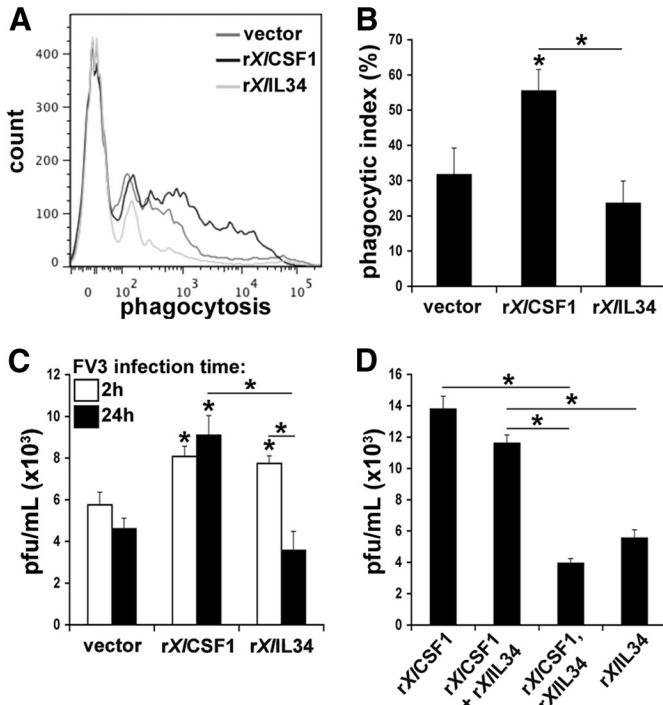
Figure 4. Tadpole rXCsf-1-pMφ are more phagocytic, whereas rXil-34-pMφ are more antiviral. (A) rXCsf-1-pMφ, rXil-34-pMφ, and vector control-elicited tadpole peritoneal phagocytes were incubated overnight (16 h) with 1 μm FITC latex beads and analyzed by flow cytometry. Cells from two individuals were pooled immediately before analysis, with six separate pools assessed per treatment group (n=6). (B) Phagocytic indexes of rXCsf-1-pMφ, rXil-34-pMφ, and control phagocyte cultures. (C) rXCsf-1-pMφ and rXil-34-pMφ exhibit similar FV3 internalization, whereas rXil-34-pMφ eliminate a significant proportion of the virus. rXCsf-1-pMφ, rXil-34-pMφ, and control phagocyte cultures were infected in vitro at a MOI of 0.5 and cells harvested for plaque assay analyses at 2 and 24 h. (D) rXCsf-1 + rXil-34-pMφ are as susceptible to FV3 as rXCsf-1-pMφ, whereas macrophages from tadpoles injected with rXCsf-1 and 36 h later, with rXil-34 (rXCsf-1, rXil-34-pMφ) are significantly more resistant to in vitro FV3 infection. rXCsf-1-pMφ, rXil-34-pMφ, rXCsf-1 + rXil-34-pMφ, and rXCsf-1, as well as rXil-34-pMφ cultures, were infected in vitro at a MOI of 0.5 for 24 h before harvesting the cells for plaque assay analyses. (B–D) Results are means ± SEM. *P < 0.05, significant difference from vector controls; *P < 0.05 (when over bars), significant differences between treatment groups denoted by the bars.
